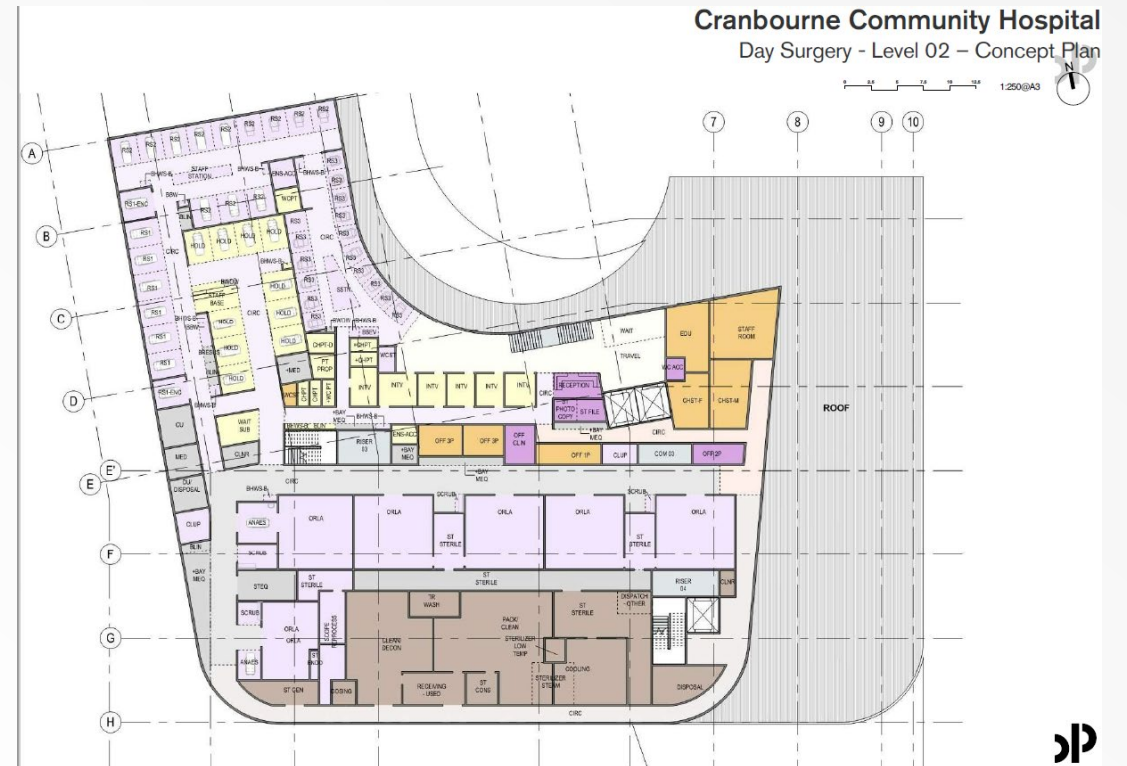
Cranbourne Day Surgery 6 theatre complex floor plan
